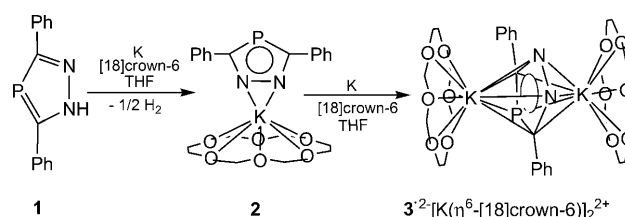
Scheme 1. Preparation of complexes 2 and 3 2- [\text{K}(\eta^6\text{-[18]crown-6})]_2^{2+} .
